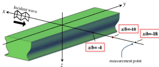
Fig. 5 Wave measurement positions
