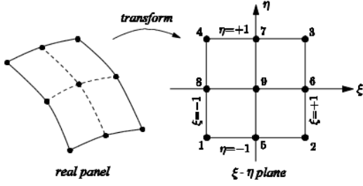
Fig. 2 Quadrilateral 9-node Lagrangian element
