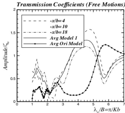
Fig. 8 Transmission coefficients of Model 1 and original model
