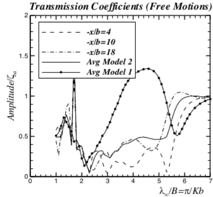
Fig. 10 Transmission coefficients of Model 1 and Model 2
