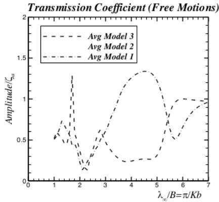
Fig. 12 Transmission coefficients of Model 1, 2 and 3
